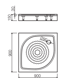
Individual shower trays
